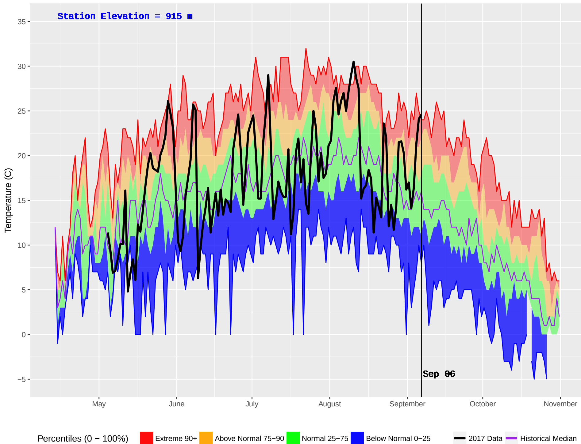
MCLEOD LAKE (153) : Historical (1990–2016) and Current (2017) Noon Temperature
