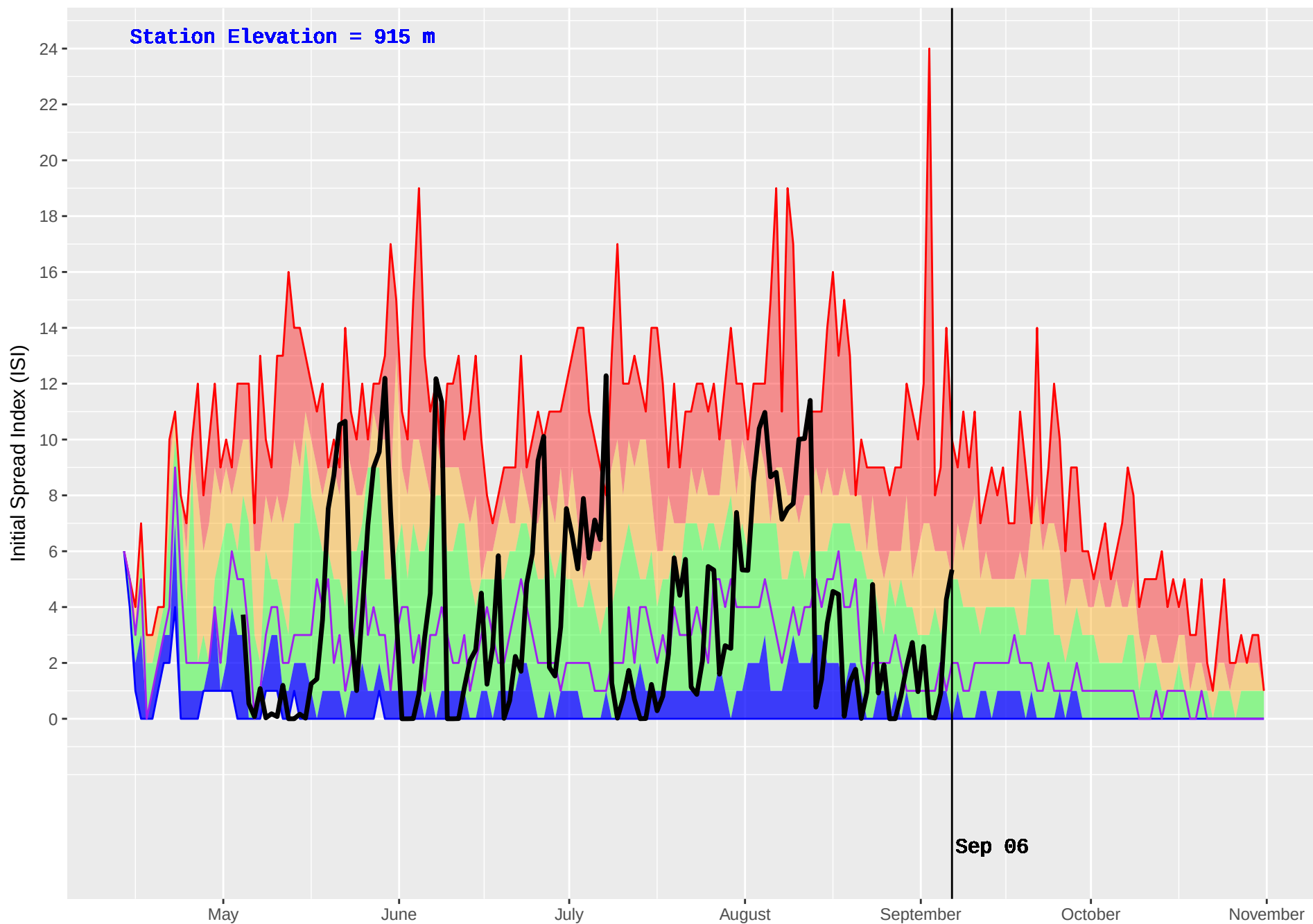
MCLEOD LAKE (153) : Historical (1990–2016) and Current (2017) Noon Initial Spread Index (ISI)
