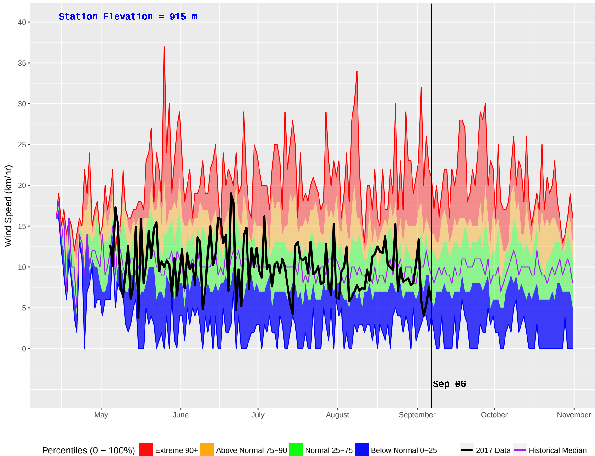
MCLEOD LAKE (153) : Historical (1990–2016) and Current (2017) Noon Wind Speed
